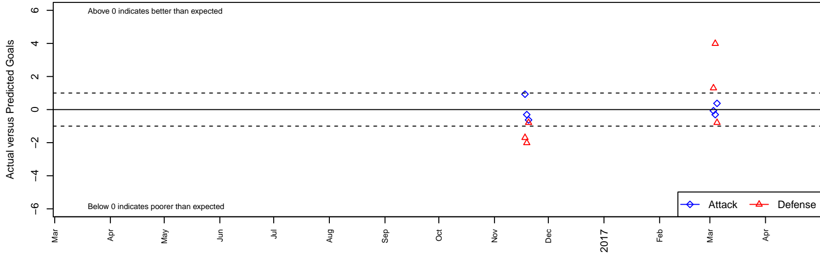
Desert Elite Red G02 Dots are actual minus expected GF (blue circles) and GA (red triangles). Blue line is smoothed change in attack strength. Red is smoothed change in defense strength.
